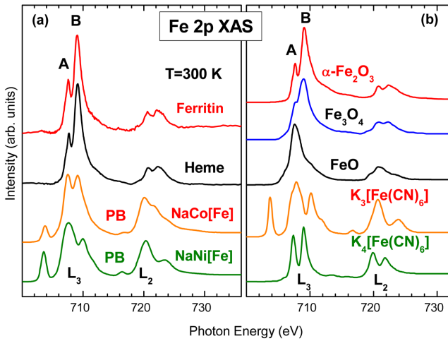
Fig. 2. (Color online) (a) Fe 2p XAS spectra of high-state ferritin, Heme, and NaM[Fe(CN) 6 ]·H 2 O (M=Co, Ni) Prussian Blue analogues. (b) Fe 2p XAS spectra of reference Fe oxides, including trivalent α-Fe 2 O 3 , mixed-valent Fe 3 O 4 , and divalent FeO. Also shown are Fe 2p XAS spectra of K 3 [Fe 3+ (CN) 6 ] and K 4 [Fe 2+ (CN) 6 ] [17] cyanide molecules.
