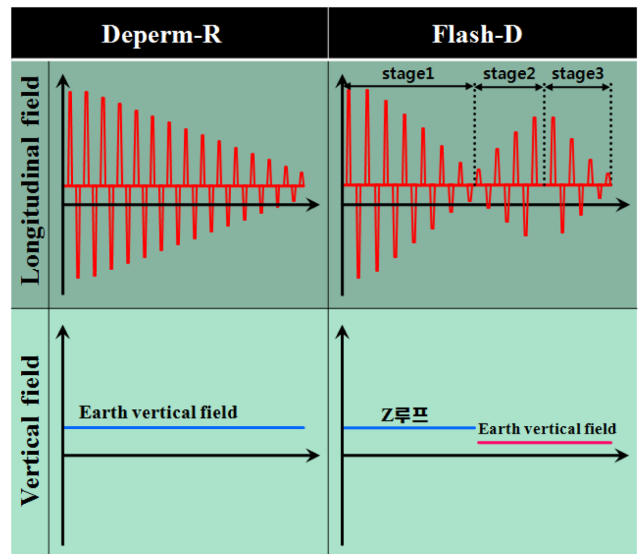
Fig. 6. (Color online) Types of the deperm protocol.
